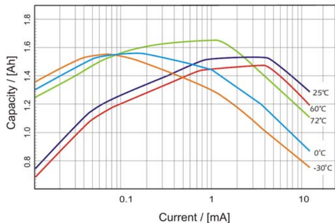
Temperature characteristics
