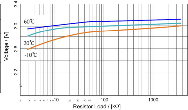
Load vs. Operating Voltage
