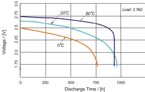
Discharges at various Temperatures
